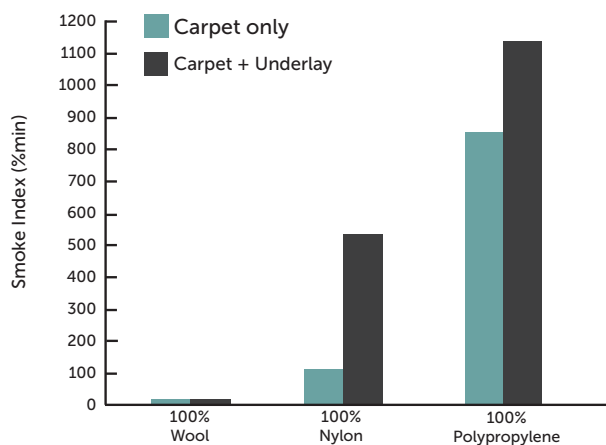
Figure 3. NBS Flooring Radiant Panel Test results for total smoke emission from Saxony carpets (Ingham 1999)
