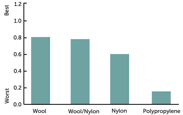
Figure 2. Energy (Radiant Panel Test) required to ignite carpets (Source: Wools of New Zealand)
