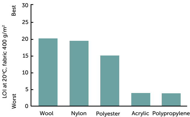
Figure 1. Limiting Oxygen Index (LOI) of common textile fibres (Source: Collie and Johnson, 1998)
