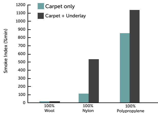
Figure 3. NBS Flooring Radiant Panel Test results for total smoke emission from Saxony carpets (Ingham 1999)
